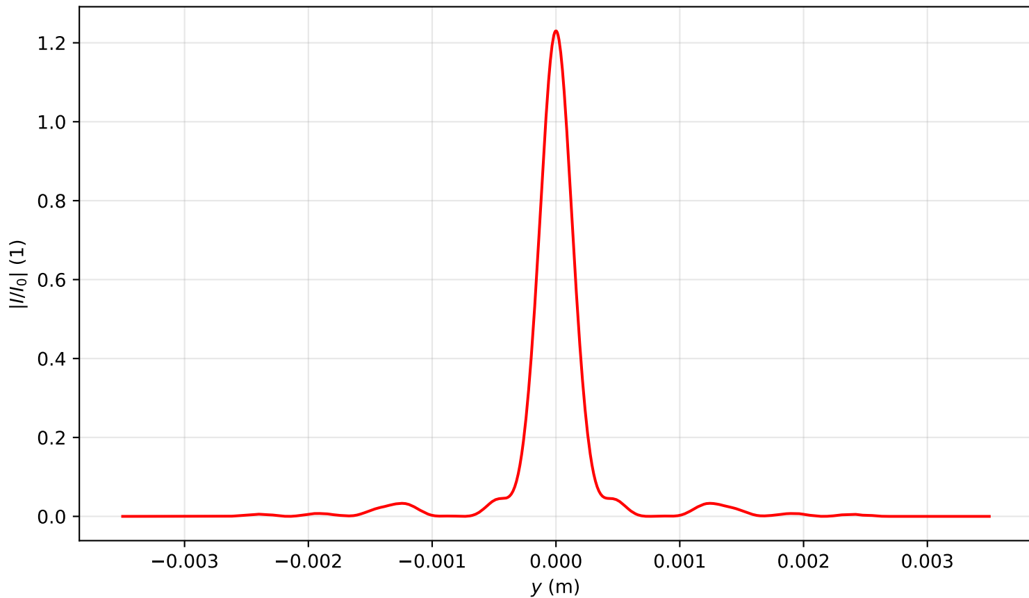
Intensity profile I(x=0, y, z=0.796)/I_0 , P_{in}=5.0P_{cr} , artificial time
